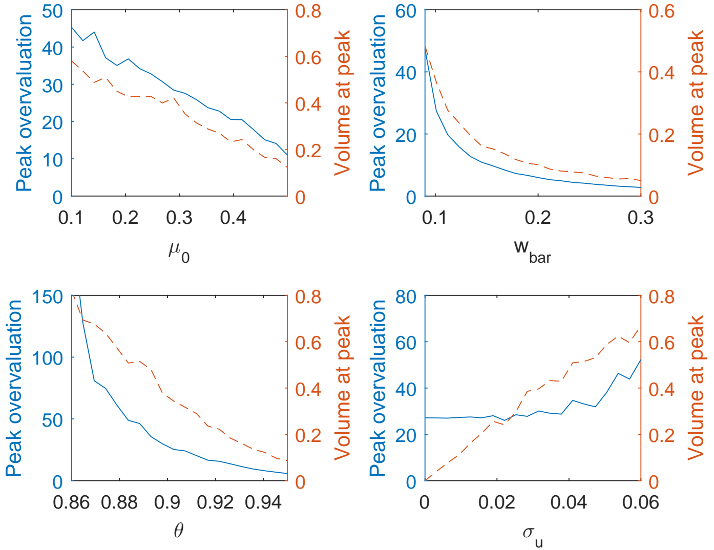
Figure 2: Comparative statics. The four graphs correspond to four model parameters: \mu_0 , \bar{w} , \theta , and \sigma_u . In each graph, the solid line plots the maximum overvaluation of the risky asset across the T = 50 dates for the same sequence of cash-flow shocks used in Figure 1; the dashed line plots trading volume on the date of peak overvaluation. The solid and dashed lines are computed by varying the value of the parameter on the horizontal axis while keeping the values of the other parameters at the benchmark levels specified in Section 2.
