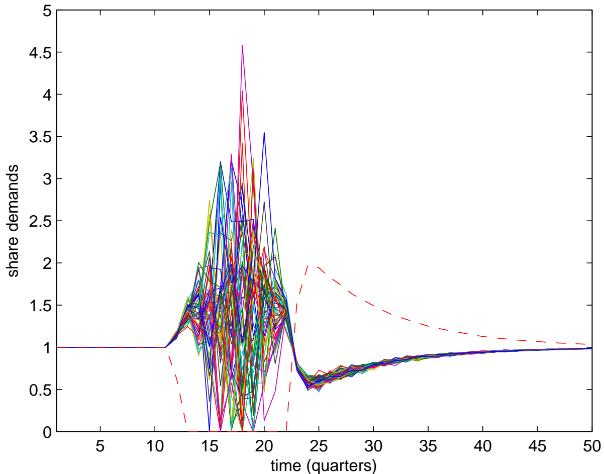
Figure 4: Share demands in a bubble. The solid lines plot the risky asset share demands of extrapolators for the following sequence of 50 cash-flow shocks: 10 shocks of zero, followed by shocks of 2, 4, 6, 6, followed by 36 shocks of zero. The dashed line plots the share demand of the fundamental traders for the same cash-flow sequence. 30% of the investors are fundamental traders; the remainder are extrapolators with an extrapolation parameter \theta of 0.9 and who also put a base weight \bar{w}_i = 0.1 on a value signal. The other parameters are D_0 = 100 , \sigma_\varepsilon = 3 , Q = 1 , \gamma = 0.1 , \sigma_u = 0.03 , and I = 50 .
