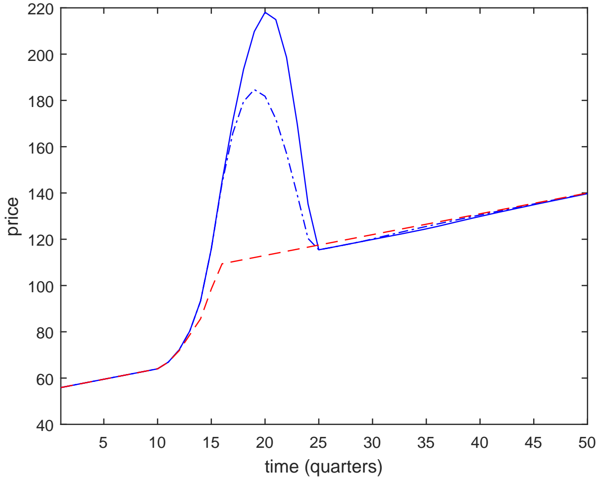
Figure 3: Price spiral. The solid line plots the price of the risky asset for the following sequence of 50 cash-flow shocks: 10 shocks of zero, followed by shocks of 2, 4, 6, 6, 12, 10, followed by 34 shocks of zero. 30% of the investors are fundamental traders; the remainder are extrapolators with an extrapolation parameter \theta of 0.9 and who also put a base weight \bar{w}_i = 0.1 on a value signal. The dashed line plots the fundamental value of the asset for the same cash-flow sequence. The dash-dot line plots the price in an economy where the extrapolators are homogeneous, placing the same invariant weight of \bar{w}_i = 0.1 on the value signal. The other parameters are D_0 = 100 , \sigma_\varepsilon = 3 , Q = 1 , \gamma = 0.1 , \sigma_u = 0.03 , and I = 50 .
