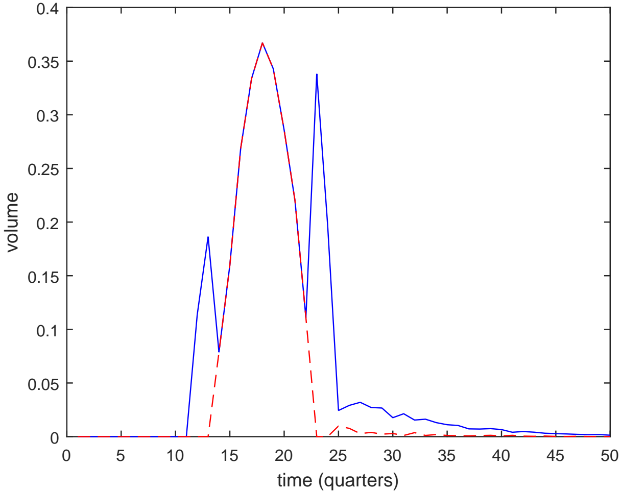
Figure 5: Volume in a bubble. The solid line plots the total trading volume in the risky asset for the following sequence of 50 cash-flow shocks: 10 shocks of zero, followed by shocks of 2, 4, 6, 6, followed by 36 shocks of zero. The dashed line plots the trading volume between the extrapolators for the same cash-flow sequence. 30% of the investors are fundamental traders; the remainder are extrapolators with an extrapolation parameter \theta of 0.9 and who also put a base weight \bar{w}_i = 0.1 on a value signal. The other parameters are D_0 = 100 , \sigma_\varepsilon = 3 , Q = 1 , \gamma = 0.1 , \sigma_u = 0.03 , and I = 50 .
