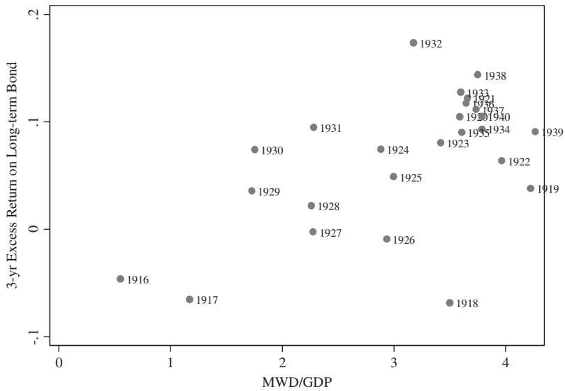
Figure 4 Bond supply and excess bond returns
