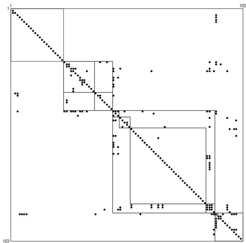
Figure 4. The Telecom DSM - architect's view.
