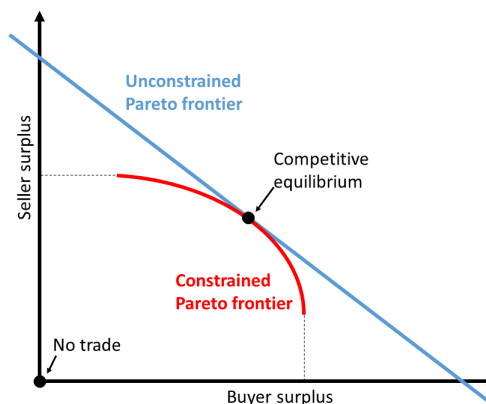
Figure 1.1: The Pareto curve without the IC and IR constraints (“unconstrained”) and with them (“constrained”).
