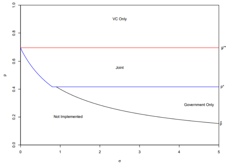
Panel A: Boundary conditions in (\sigma, p) space, with increased PB .
