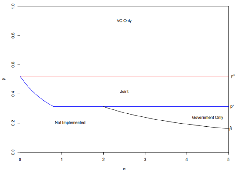
Panel B: Boundary conditions in (\sigma, p) space, with increased beta.
