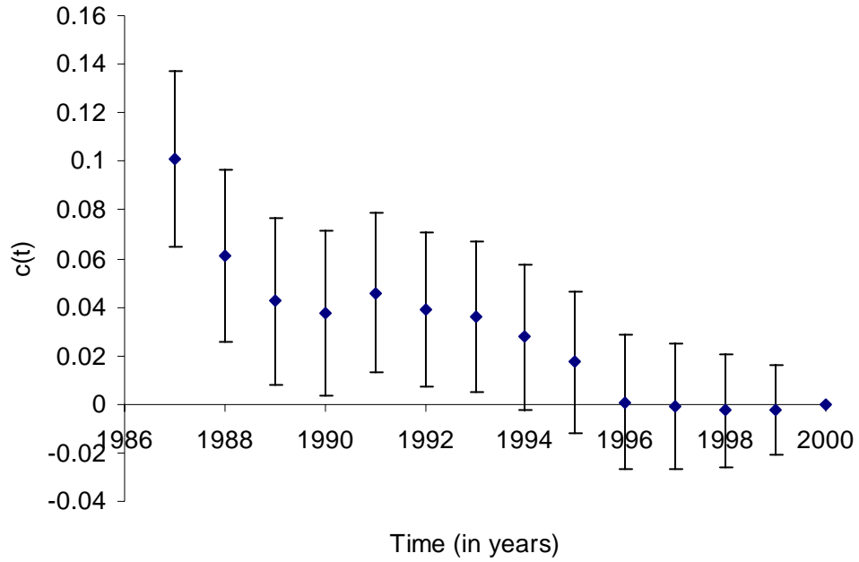
Figure 2: Plot of time-specific fixed effects c_t for model (2) (the error bars show intervals of 2 \times standard error)
