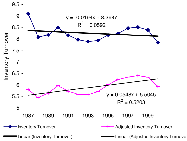
Figure 4: Plot of Inventory Turnover and Adjusted Inventory Turnover for Ruddick Corp.
