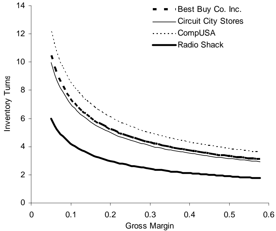
Figure 3: Tradeoff curves between inventory turnover and gross margin estimated for the four consumer electronics retailers in Figure 1
